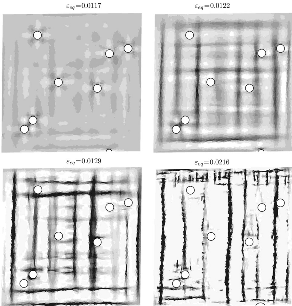
Figure 12. Maps of plastic strain rate ( s^{-1} ) in a random distribution of particles ( f=2\% ) loaded in shear at different strain levels. The shearing axes are horizontal and vertical, respectively.
