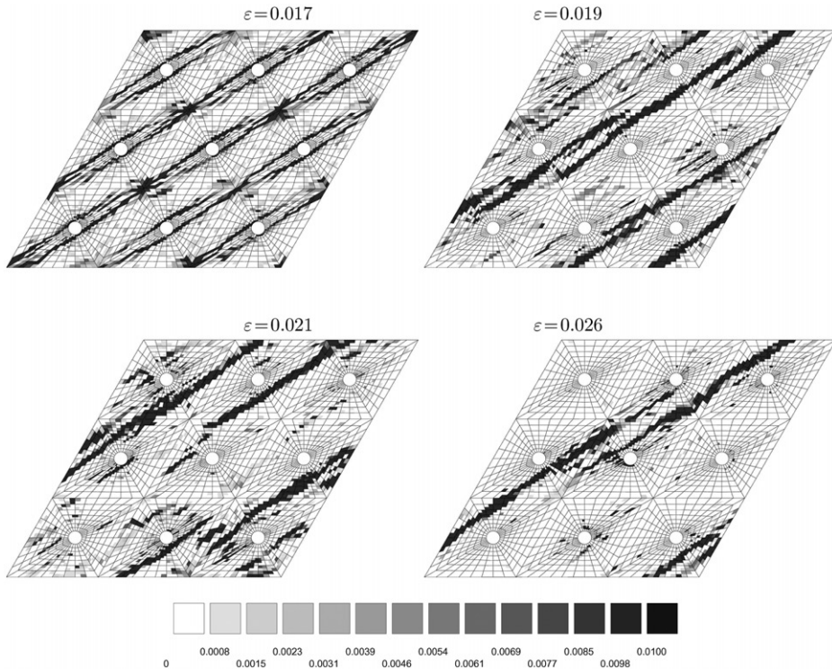
Figure 9. Maps of plastic strain rate ( \text{s}^{-1} ) in the 9-inclusion unit cell with the periodic distribution of particles for f = 2\% , at different mean strain levels indicated by symbols on the macroscopic curve of Figure 6a. The tensile axis is vertical.
