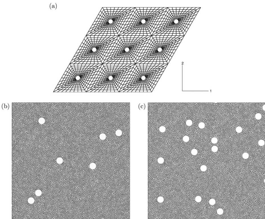
Figure 8. FE meshes for periodic and random distributions of particles: (a) periodic mesh with 9-inclusion unit cell with f=2\% , (b) mesh with a random distribution of particles with f=2\% , (c) mesh with a random distribution of particles with f=5\% . The axes indicated in (a) are also valid for (b) and (c).
