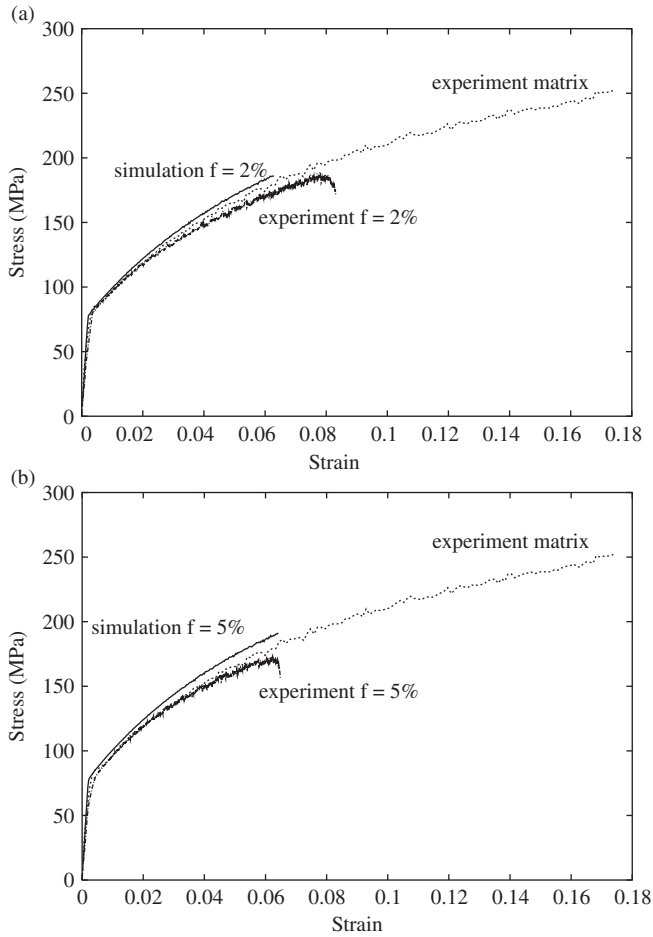
Figure 7. Comparison of the experimental and simulated stress–strain curves between the parent Al-3% Mg alloy and the AA5754 MMC at room temperature at \dot{\epsilon} = 6.2 \times 10^{-3} \text{ s}^{-1} with: (a) f=2\% , (b) f=5\% .
