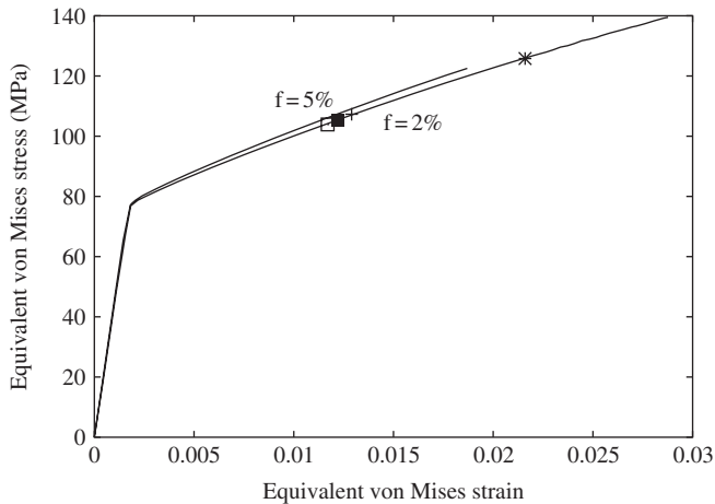
Figure 10. Influence of particle volume fraction f on the computed stress–strain curves for the AA5754 MMC in tension at \dot{\epsilon} = 6.2 \times 10^{-3} \text{ s}^{-1} . Simulation with a random distribution of particles. The symbols indicate the strain levels corresponding to the plastic strain rate maps given in Figure 11.
