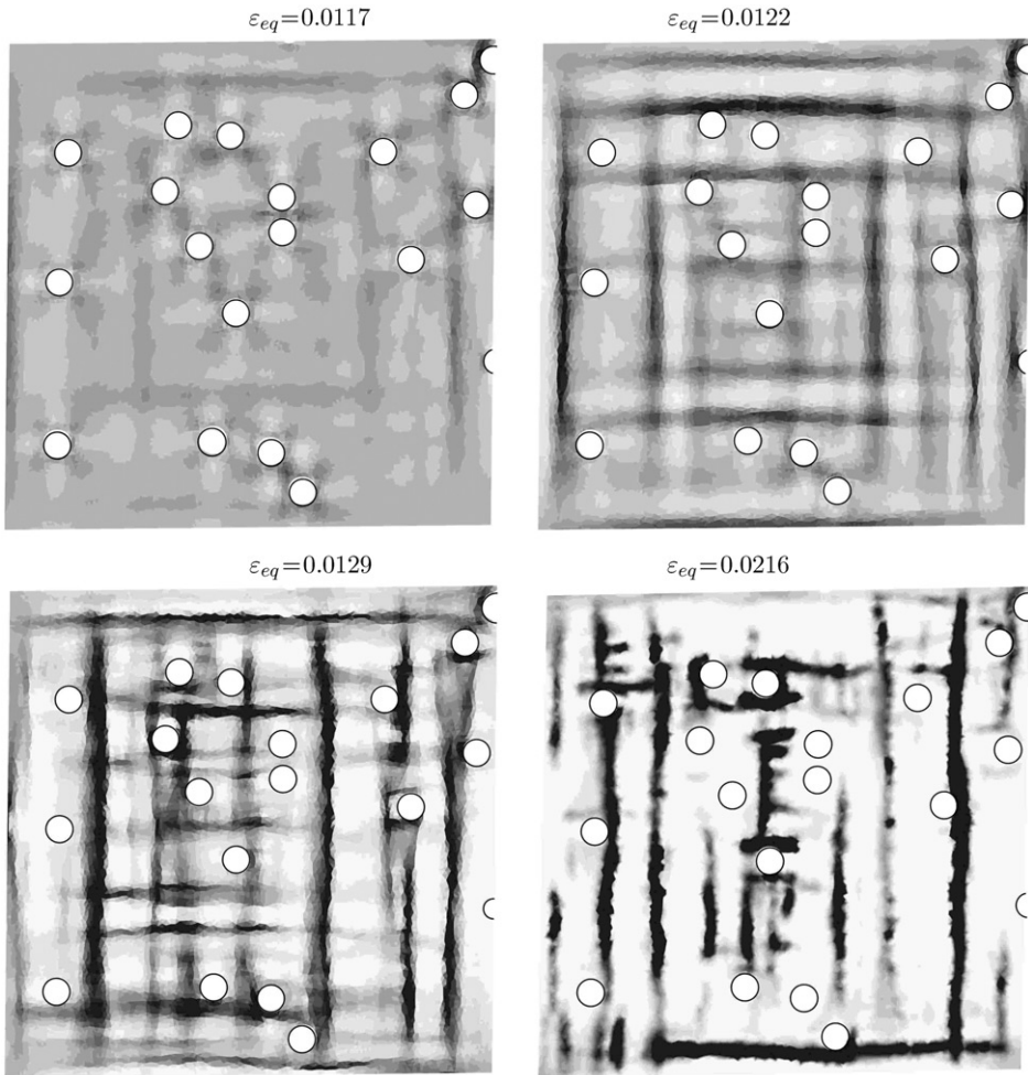
Figure 13. Maps of plastic strain rate ( \text{s}^{-1} ) in a random distribution of particles ( f=5\% ) loaded in shear at different strain levels.
