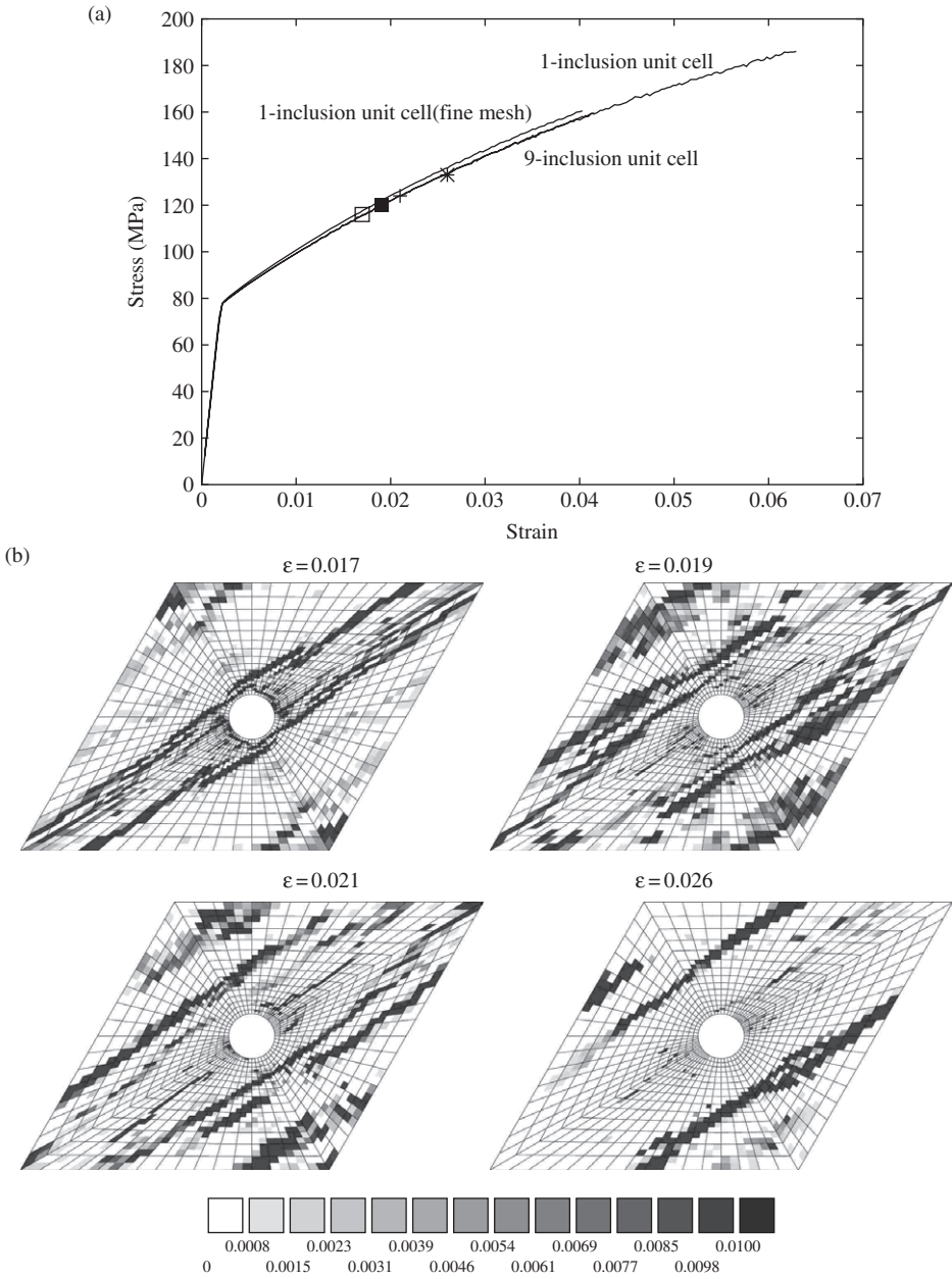
Figure 6. (a) Influence of mesh refinement and of the choice of the unit cell on the stress–strain curves for the AA5754 MMC with f=2\% at \dot{\epsilon} = 6.2 \times 10^{-3} \text{ s}^{-1} ; (b) maps of plastic strain rate (in \text{s}^{-1} ) in the 1-inclusion cell ( f=2\% ), at different mean strain levels which are indicated on the macroscopic curve (a).
