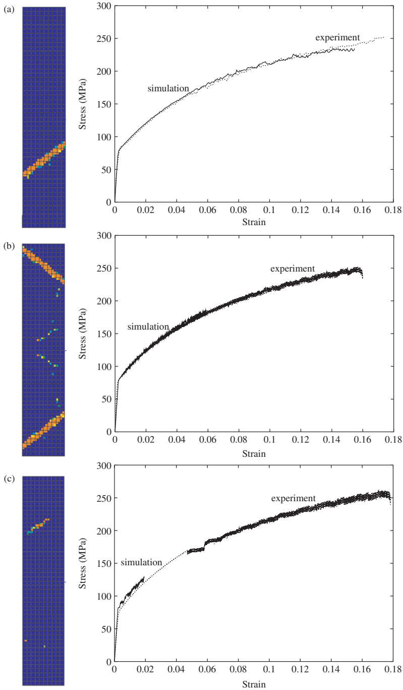
Figure 3. (Color online). Comparison of the experimental and simulated stress–strain curves for the parent Al-3% Mg alloy at different applied strain rates: (a) \dot{\epsilon} = 6.2 \times 10^{-3} \text{ s}^{-1} , (b) \dot{\epsilon} = 1.1 \times 10^{-4} \text{ s}^{-1} , (c) \dot{\epsilon} = 1.1 \times 10^{-5} \text{ s}^{-1} . The experimental curves are in dotted lines. For each strain rate, a typical distribution of the plastic strain rate \dot{\epsilon} in the tensile plate is given. The red colour corresponds to strain rates five times higher than the overall prescribed strain rate.
