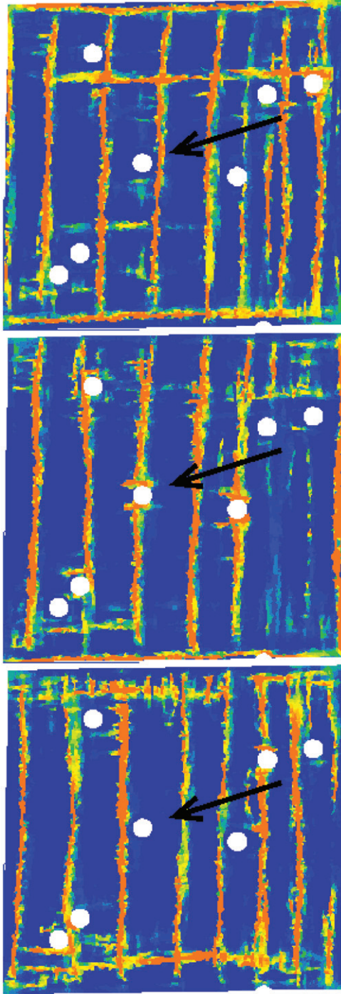
Figure 14. (Color online). Overcoming of obstacles by the PLC band in a MMC with f=2\% subjected to shear loading conditions. The arrow indicates the location of a particle for which the scattering of the band is clearly visible when it hits the obstacle.
