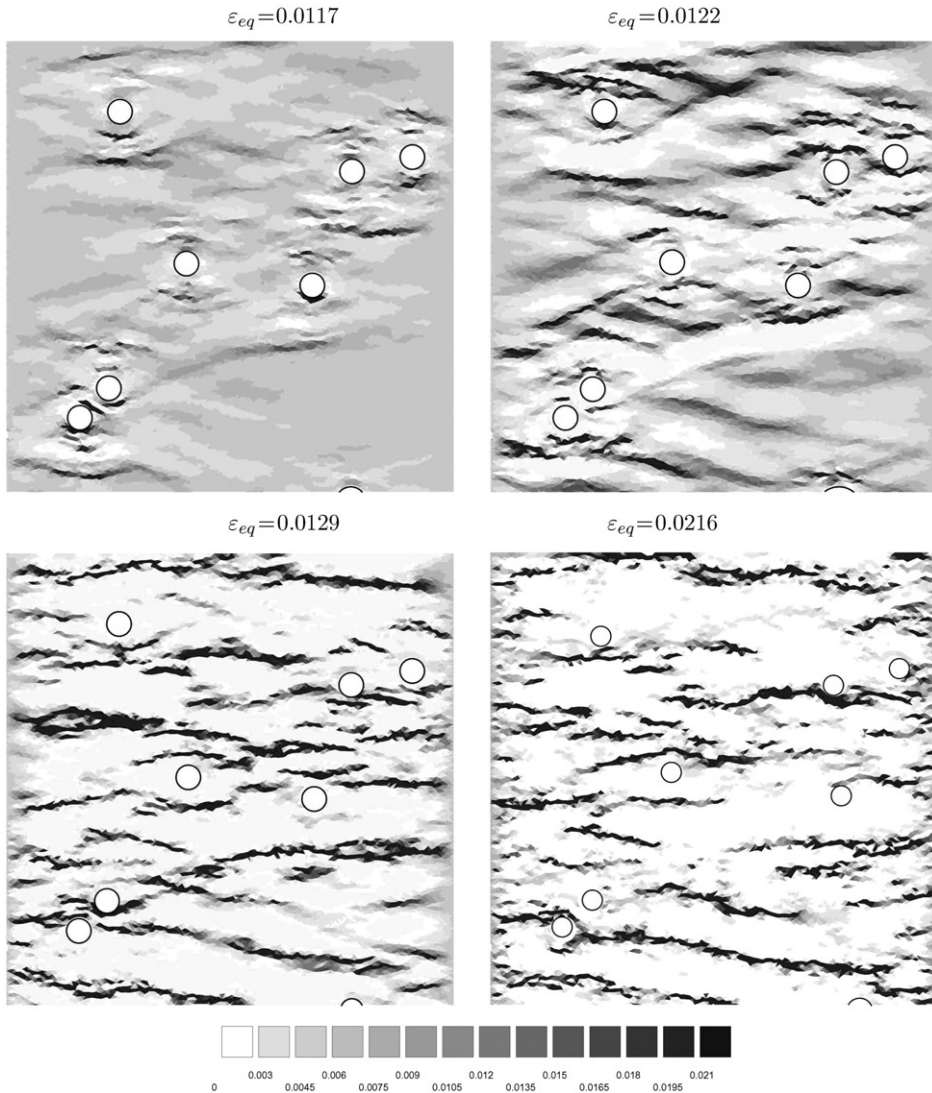
Figure 11. Maps of plastic strain rate ( s^{-1} ) in a random distribution of particles ( f=2\% ) loaded in tension at different strain levels indicated by symbols on the macroscopic curve of Figure 10. The tensile axis is vertical.
