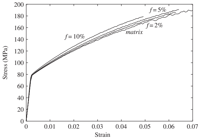
Figure 4. Influence of the volume fraction of particles on the computed stress–strain curves at \dot{\epsilon} = 6.2 \times 10^{-3} \text{ s}^{-1} for the AA5754 MMC. From the lower to the upper curves we have successively: the parent Al-3% Mg alloy, the AA5754 MMC with f=2\% , the AA5754 MMC with f=5\% , and the AA5754 MMC with f=10\% .
